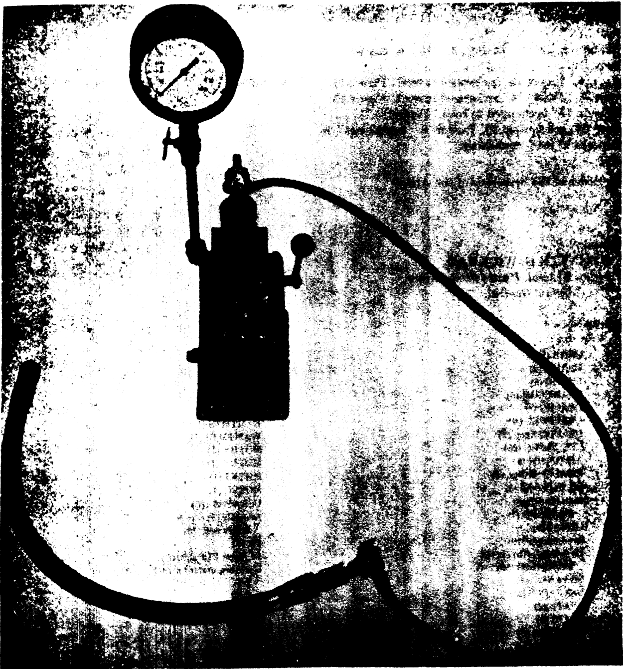
Figure 13. M8 hose attached to test set for hydrostatic test.
